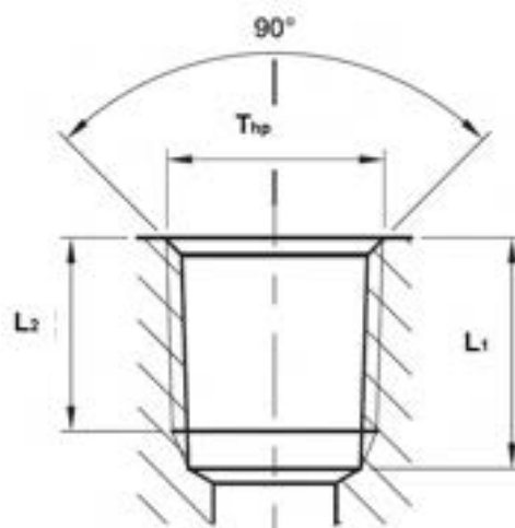
Port (Parallel Thread)
