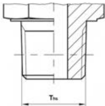
BSPT Tapered Thread
