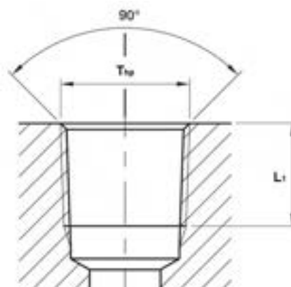
Port (Tapered Thread
