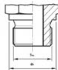
Sealing: Sealing washer DIN 7603 (e.g. copper)
